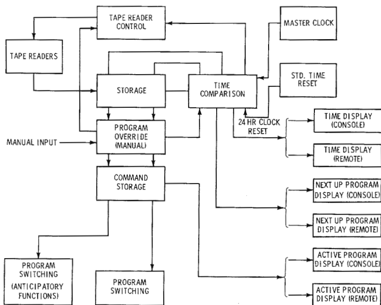
Fig. 1. Typical computer block diagram.
