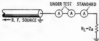
Fig. 1. Series meter current method.
