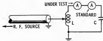
Fig. 2. Tuned L and C test method.
