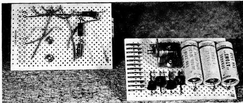
Fig. 5. Construction of power supply.
