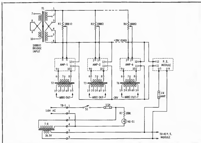
Fig. 6. Diagram of chassis wiring arrangement.
