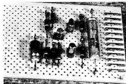
Fig. 3. Board-constructed amplifier unit.
