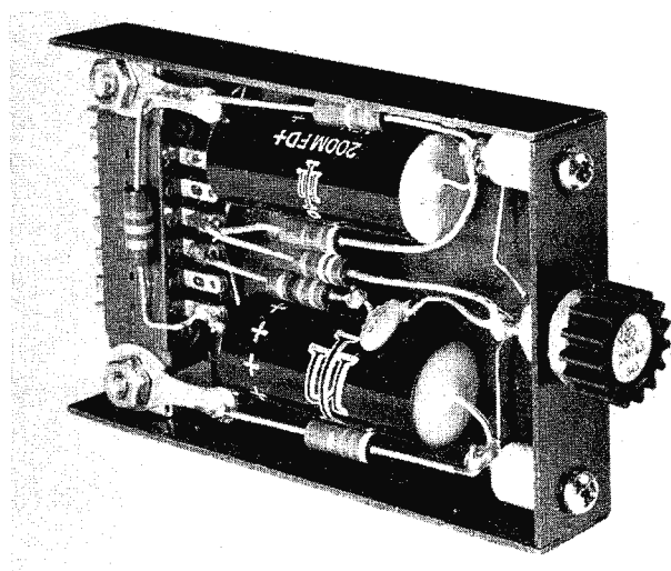
Fig. 3. Typical line driver input amplifier.
